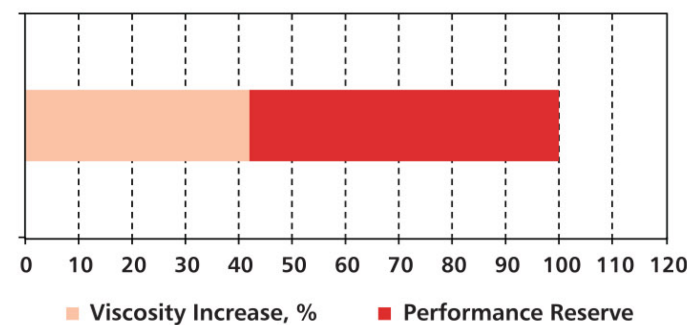
Sequence IIIG Oxidative Stability Control
